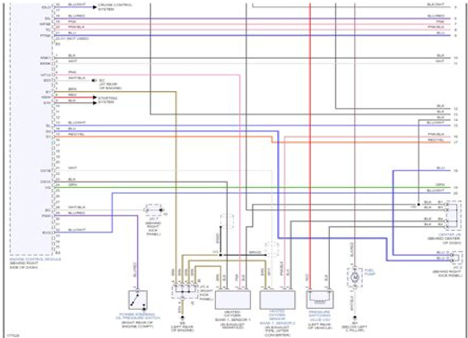
Fig 1: 1.8L, Engine Performance Circuit (1 of 3)
