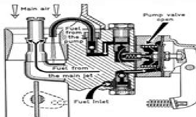
Fig. 34 "Slide" pump with ball valve (pump 73)
