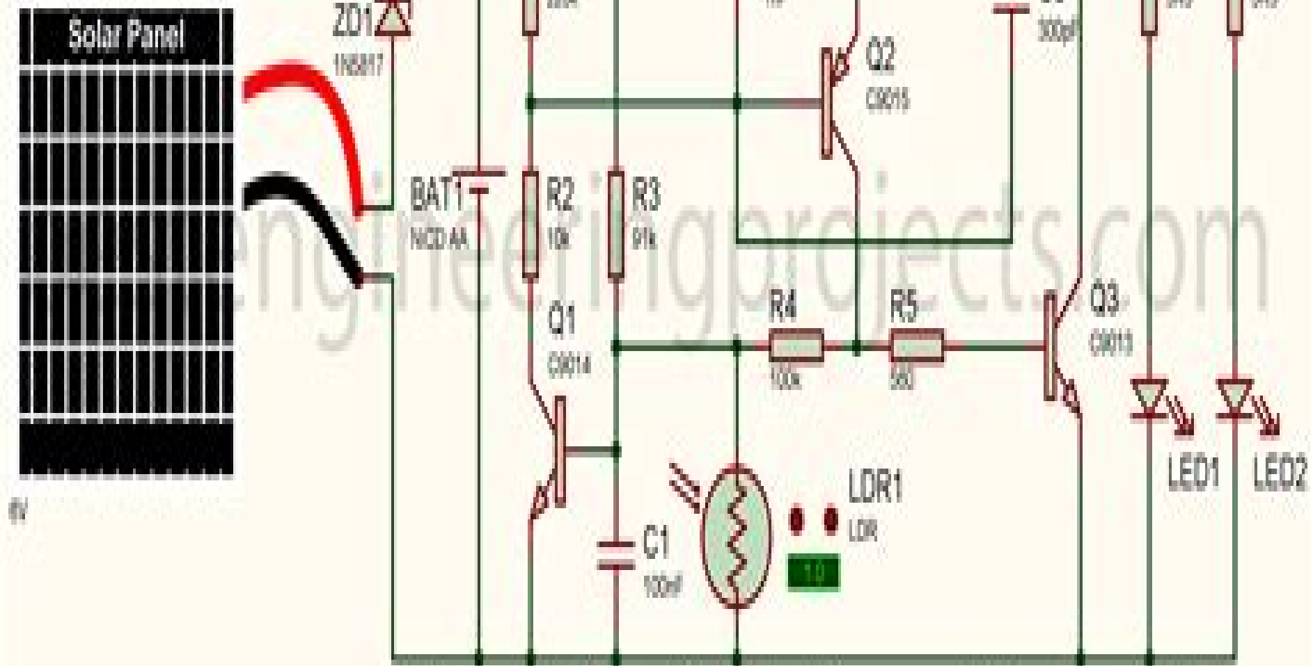
Figure 1: Circuit Solar Powered Garden Light
