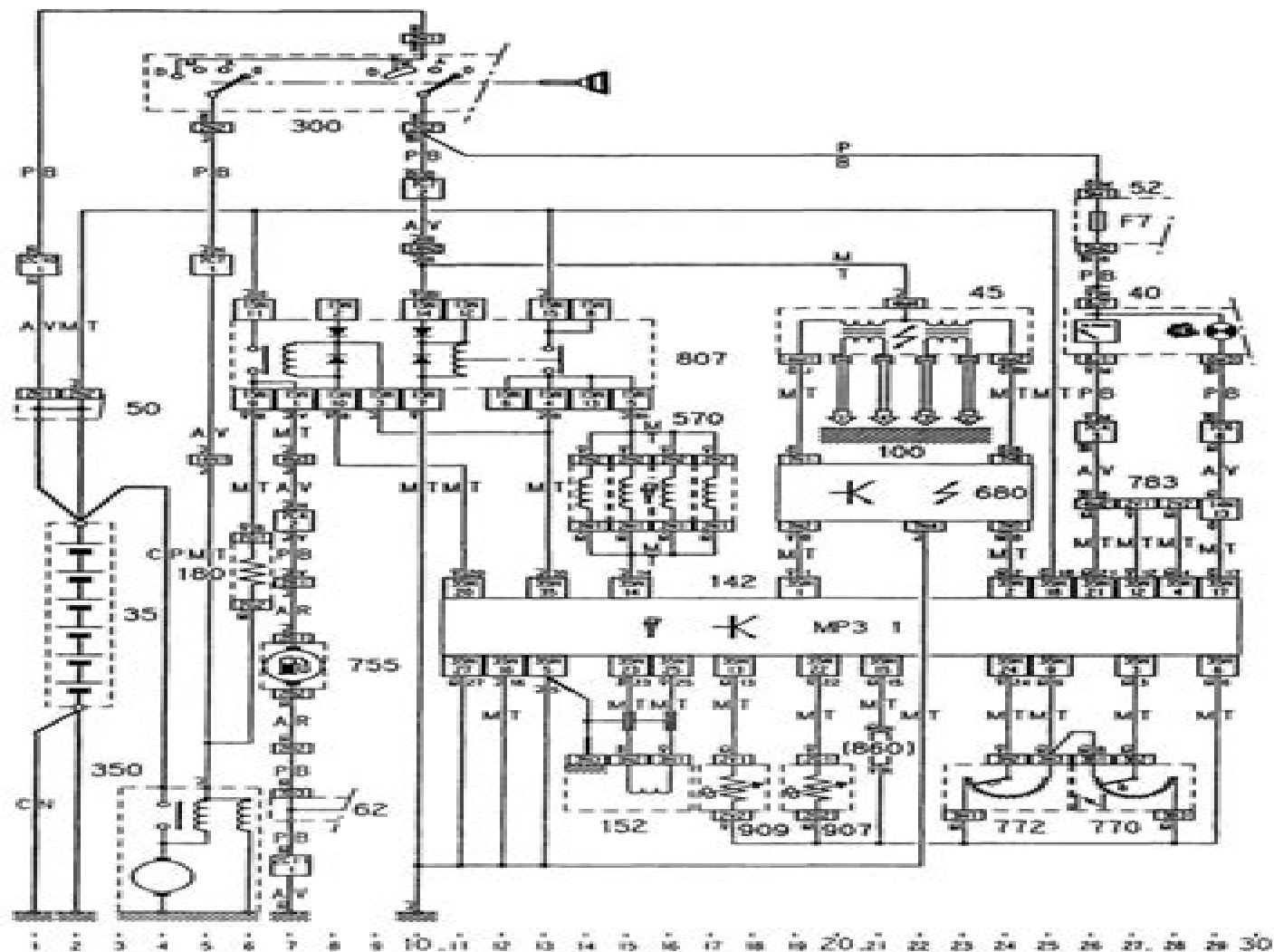
Engine electrical systems - 1995 cc non-catalyst (D6E/XU9JA, K)
