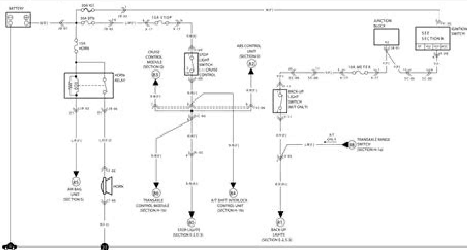
F-28 HORN SWITCH (1)
