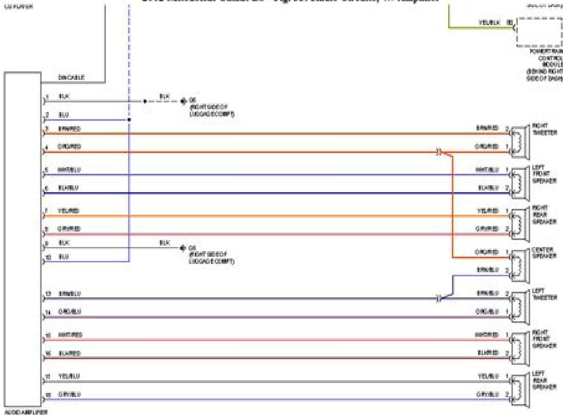
2002 Mitsubishi Galant ES - Fig. 35: Radio Circuits, W/ Amplifier
