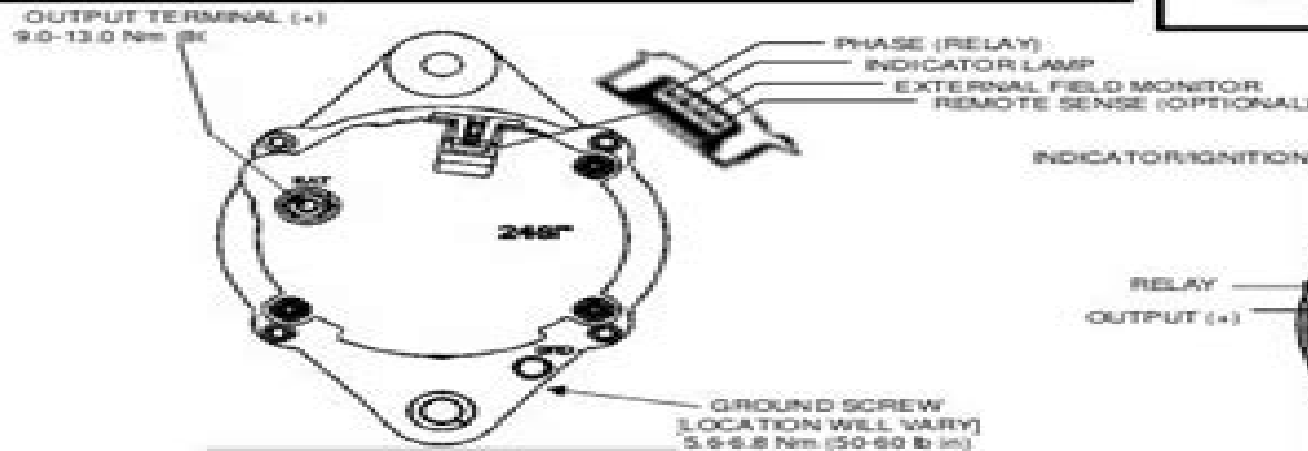
24SI ALTERNATOR
