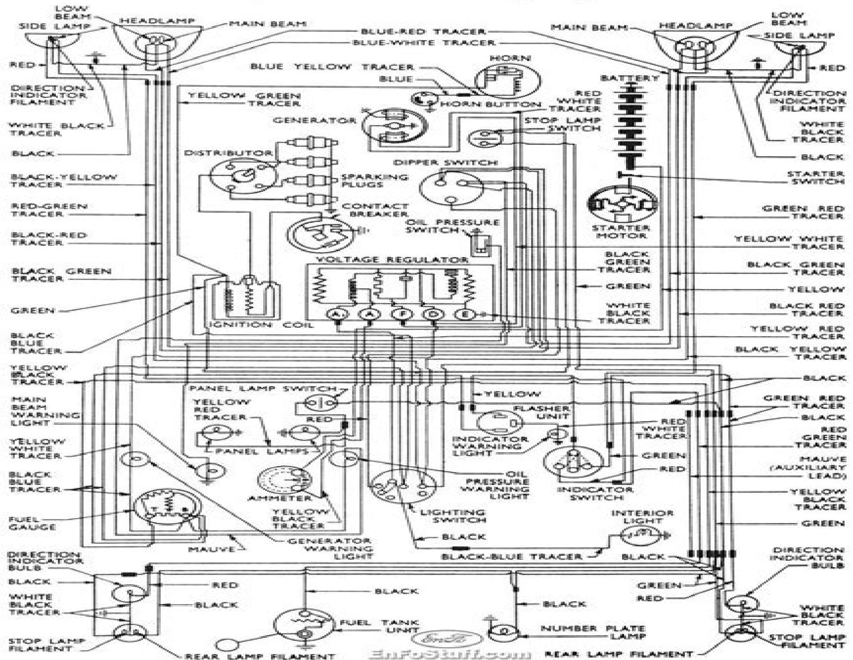
Chassis wiring diagram, Anglia 1953-57.
