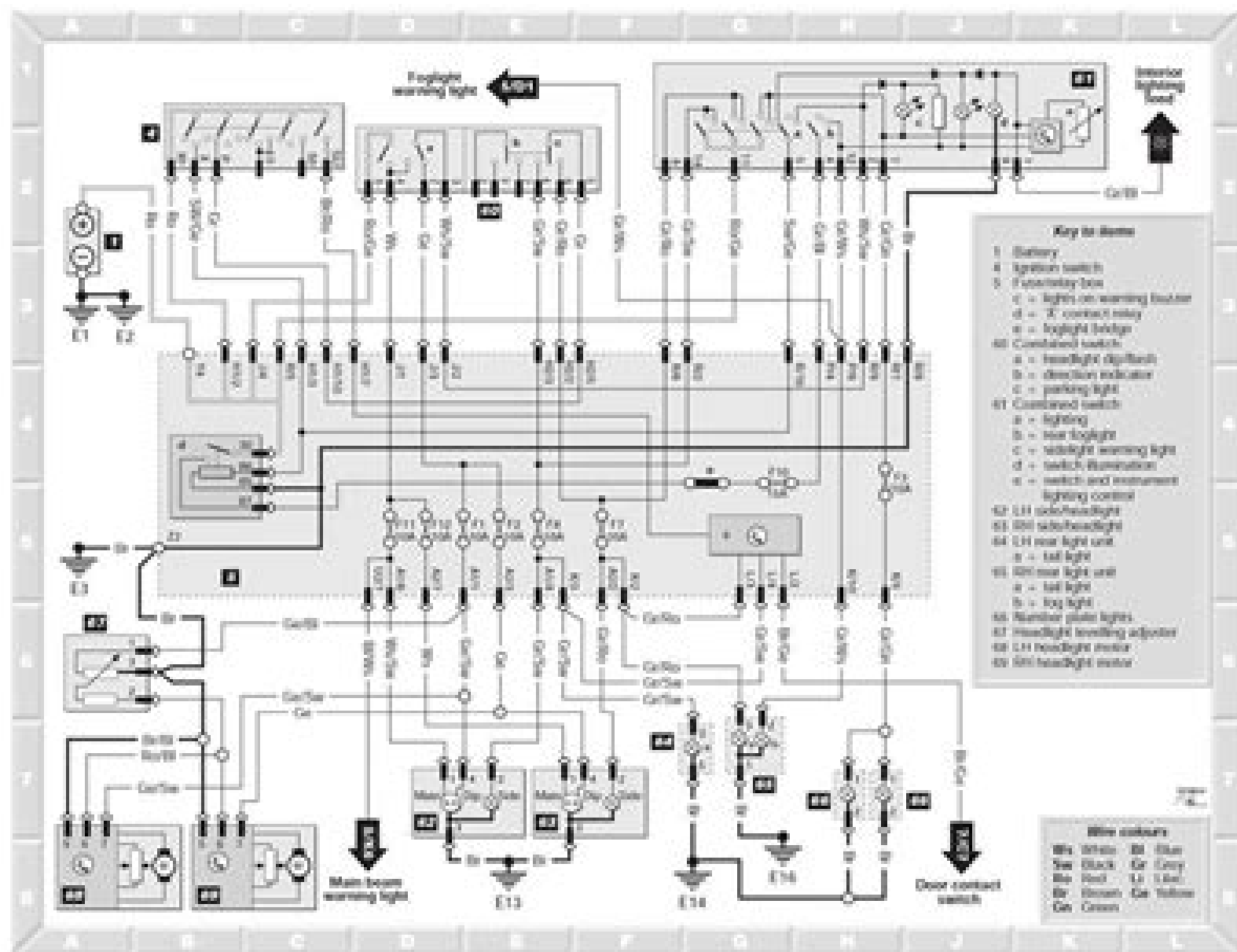
Diagram 6 : Side, tail, number plate, head and foglights, headlight levelling - models up to 1999
