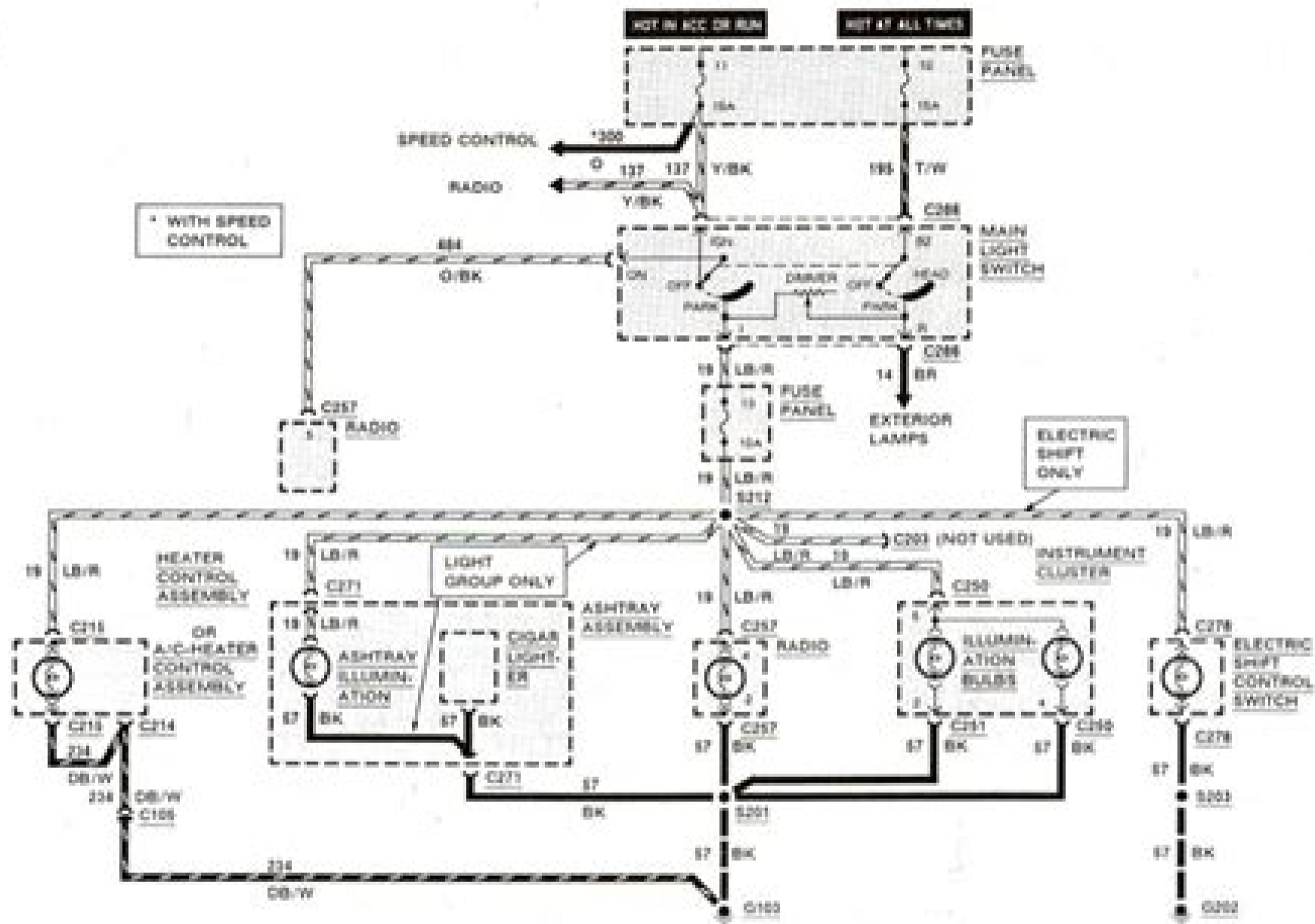
Instrument panel lights – 1990 on (typical)
