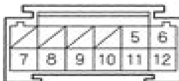
Terminal side of male terminals
