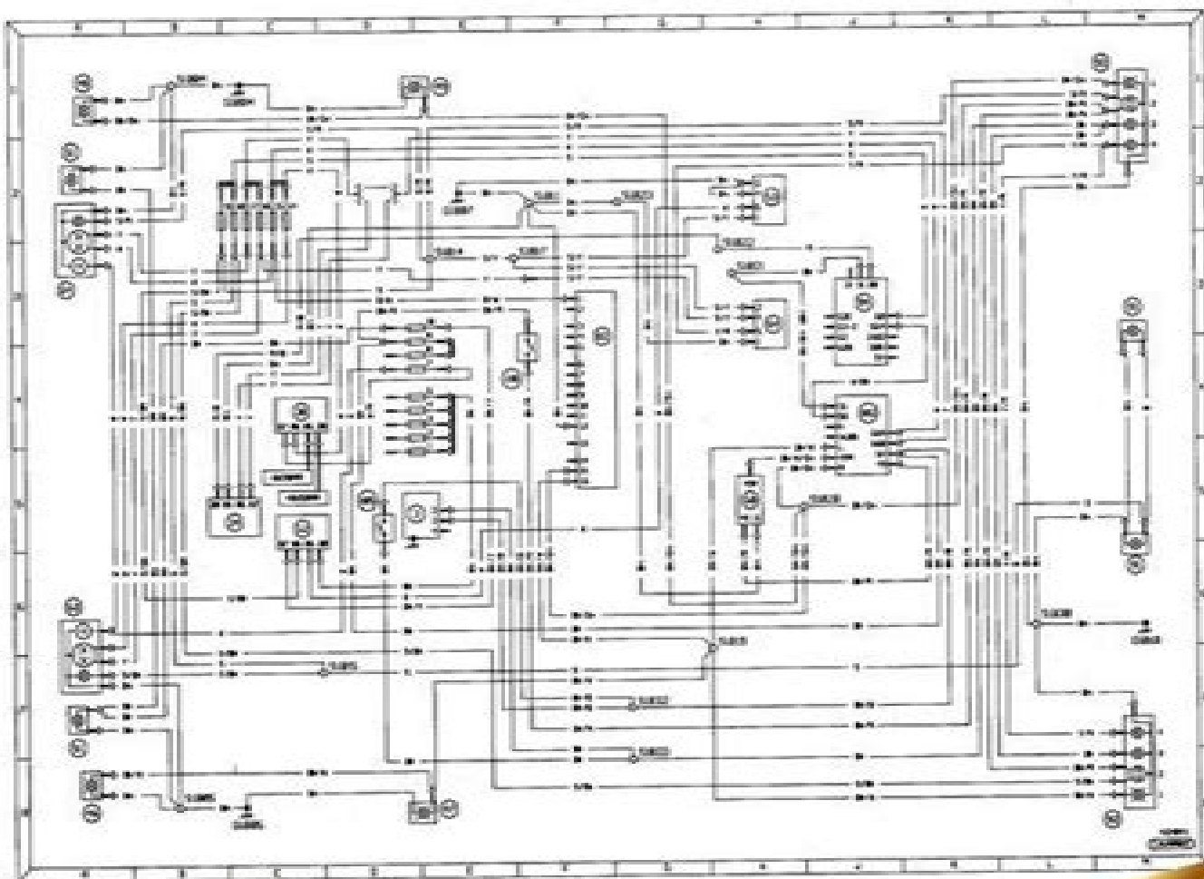
Diagram 2. Exterior lighting. Models up to 1987
