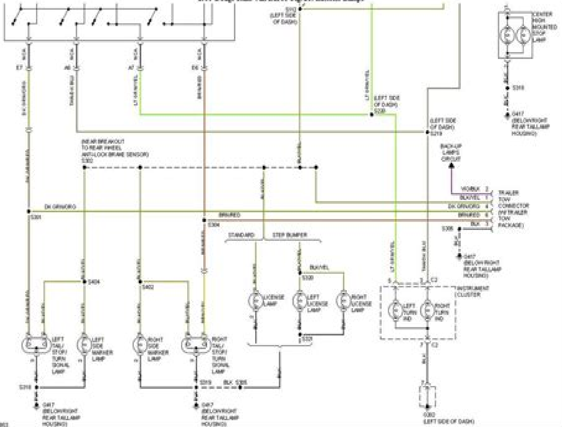
1999 Dodge Ram Van B1500-Fig. 30: Exterior Lamps
