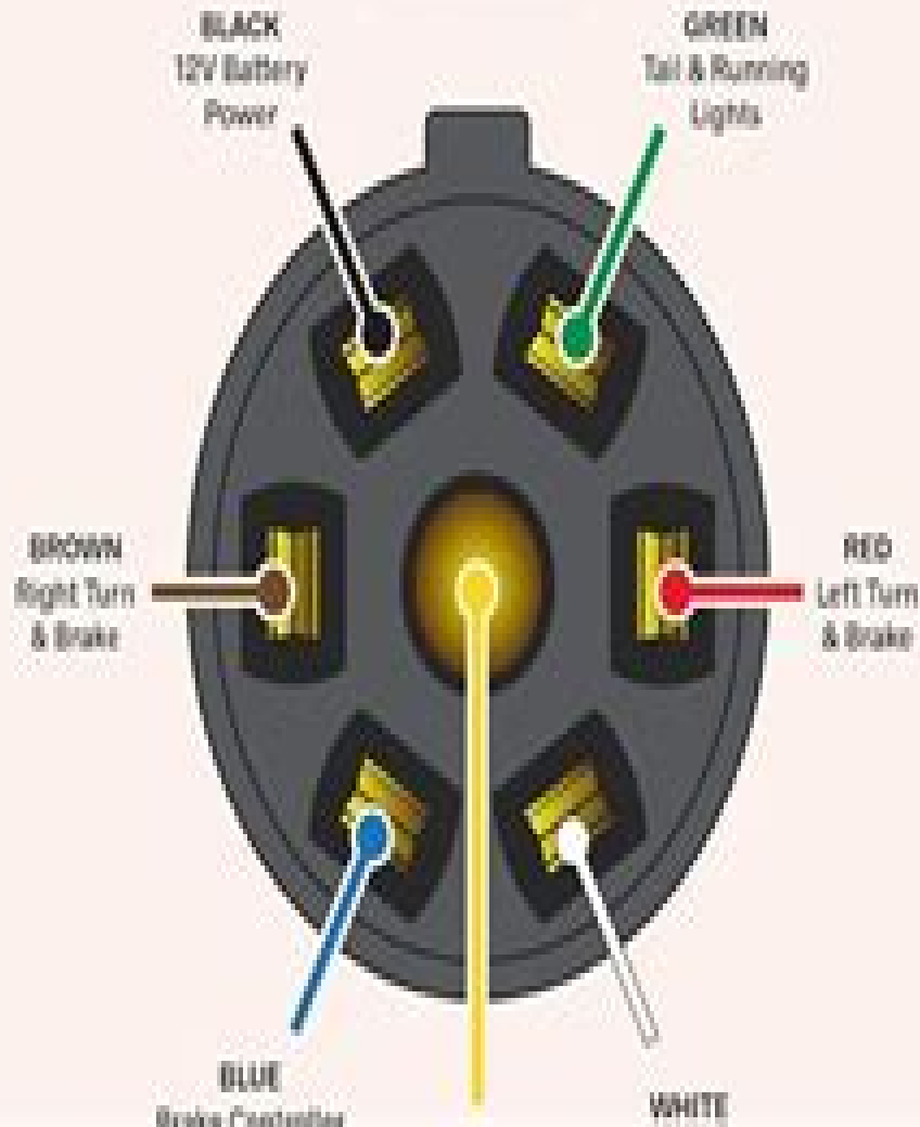
Plug Side
