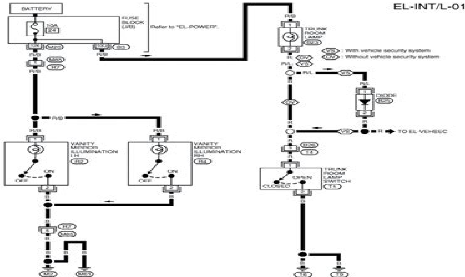
Wiring Diagram — INT/L —
