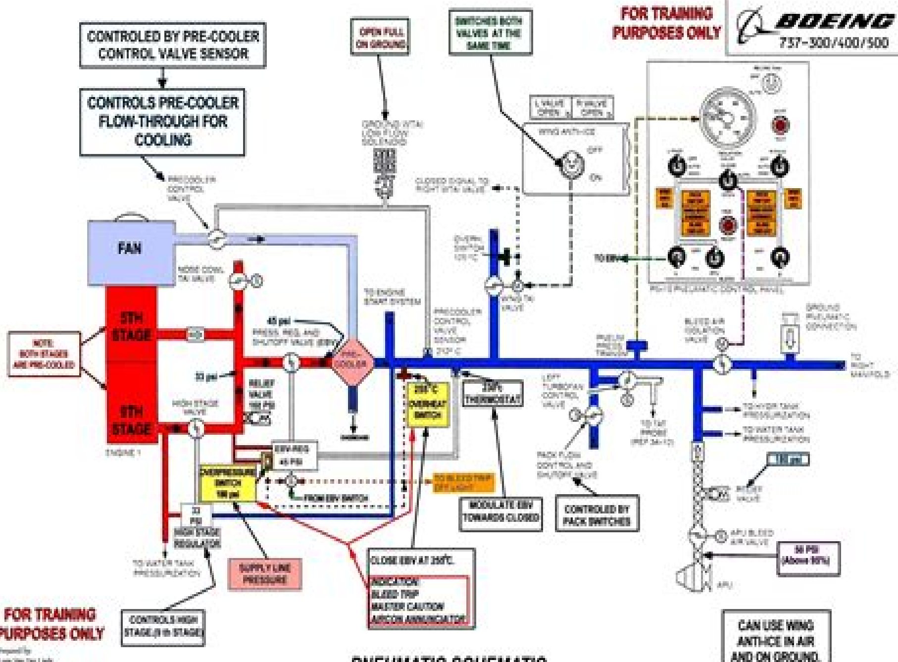
PNEUMATIC SCHEMATIC
