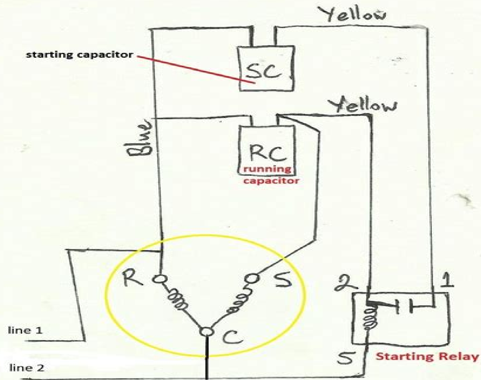
compressor with starting capacitor
