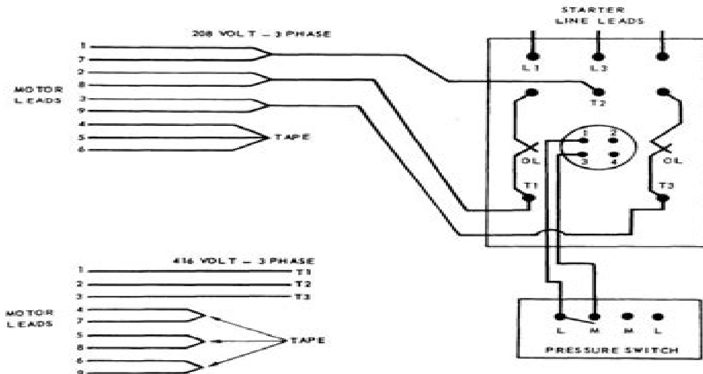
Figure 3.2. (Added) Wiring diagram (Model OEH-34-60-ENG-4).
