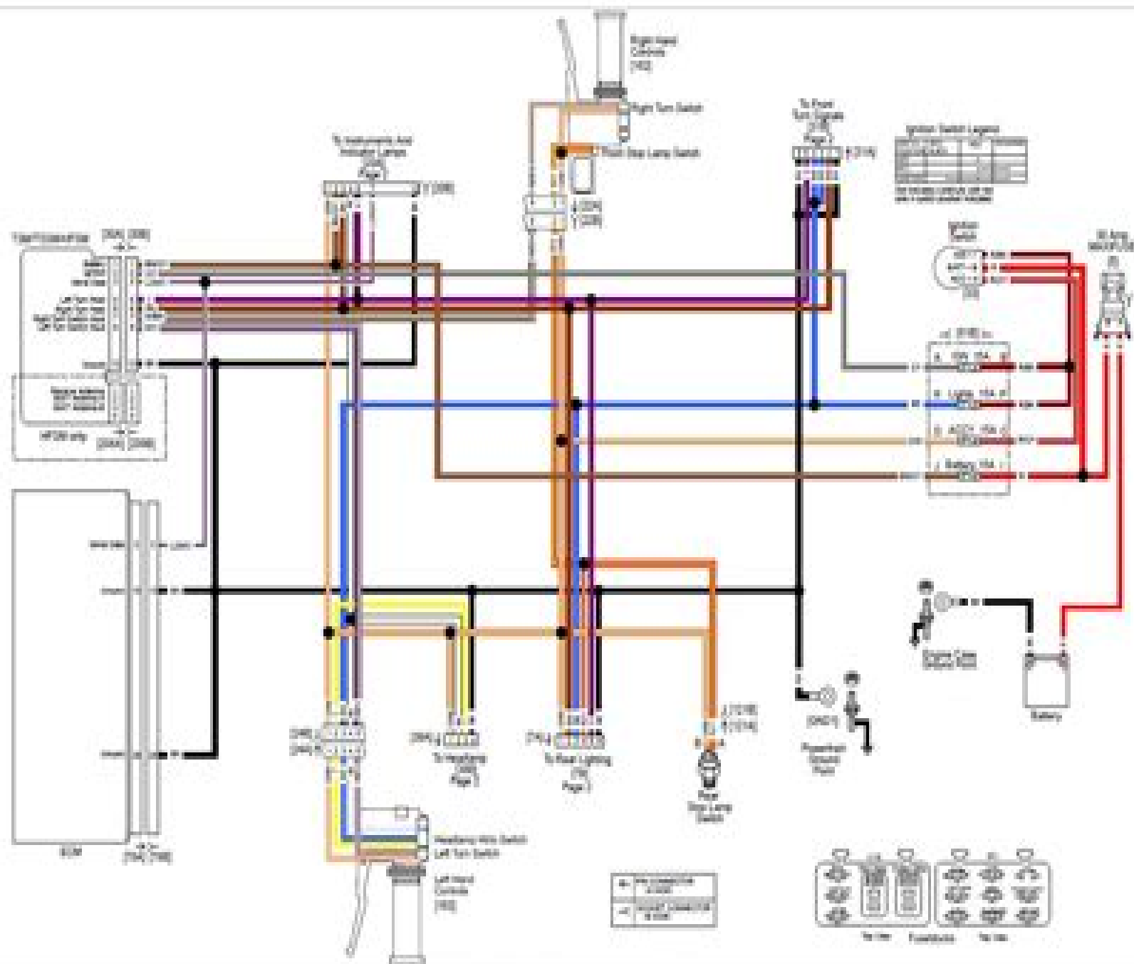
Figure B-14. Lights (1 of 2) (2009 Sprinter 2500 and 3500 Models)
