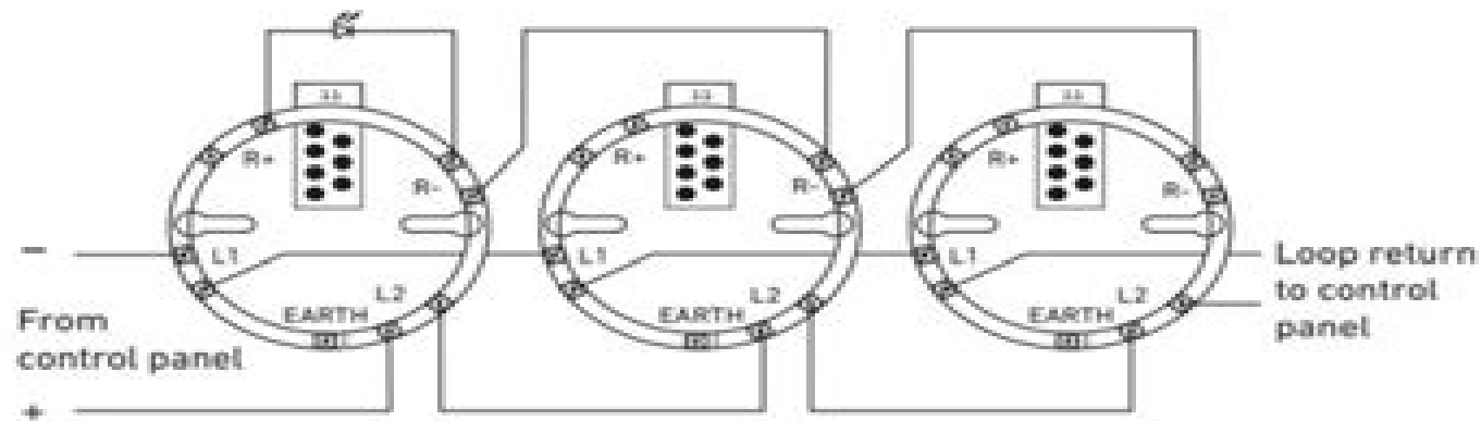
Schematic wiring diagram of an analogue addressable detector circuit with a common remote LED
