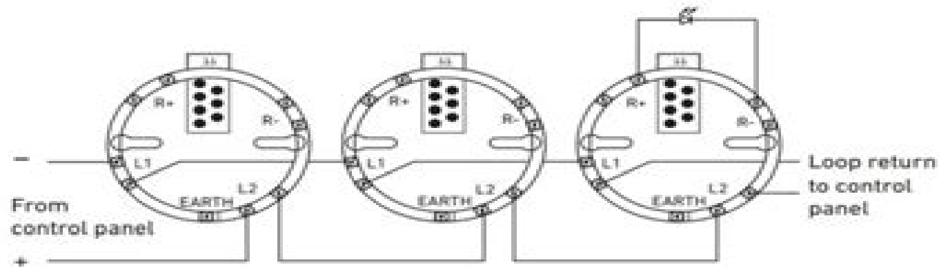
XPERT7 Intelligent Mounting Base - schematic wiring diagram
