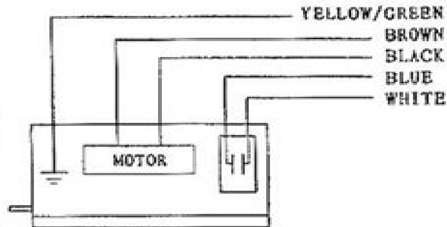
Fig7: Wiring with auxiliary switch
