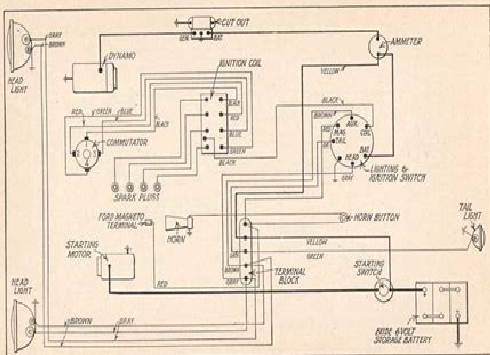
Fig. 87. Wiring Diagram with Cutout on Dash
