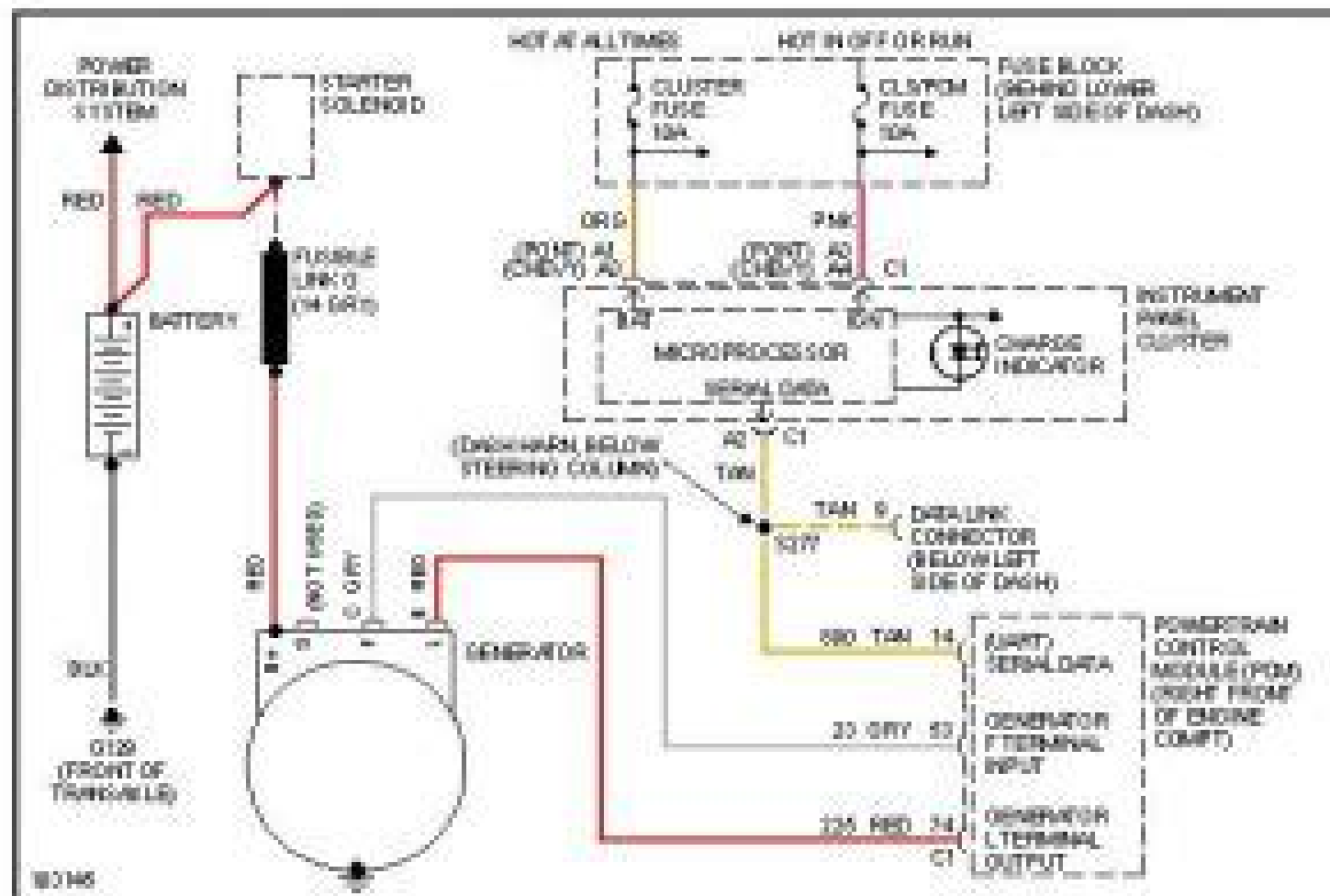
1998 Pontiac Sunfire SE-Fig. 37: Charging Circuit
