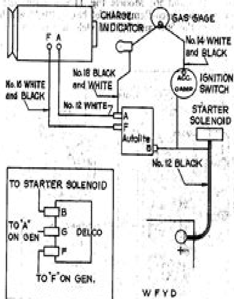
GENERATOR CIRCUIT
