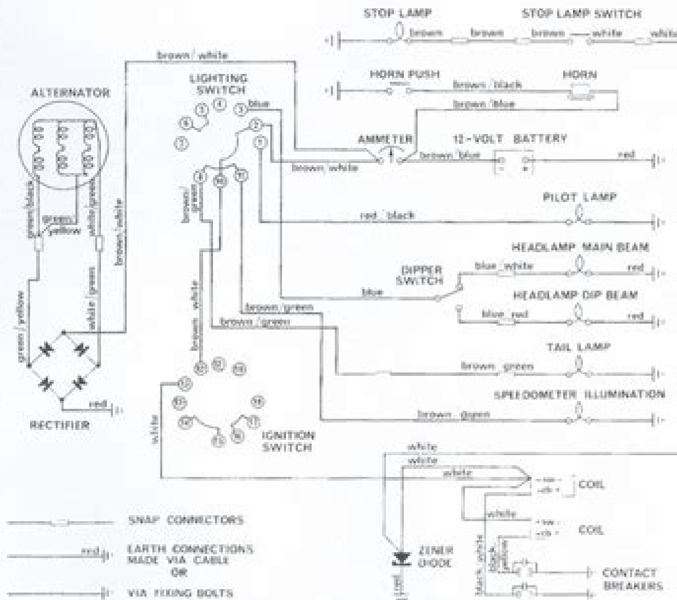
Fig. H34. Wiring diagram—Coil ignition 12 volt models with nacelle from engine number DU2M75 Note. The main beam warning lamp (where fitted) is connected to the headlamp main beam wire (blue/white) by a double snap connector. The ignition warning lamp is connected to an ignition coil by a white wire incorporated in the wiring harness.
