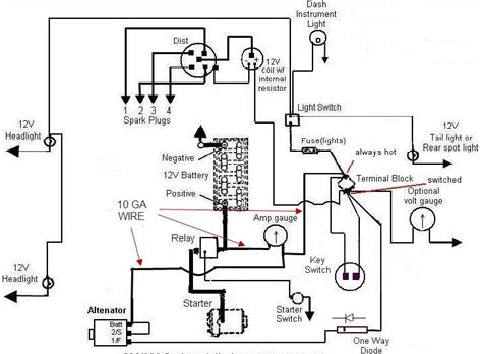
600/800 3 wire w/ diode 12V Conversion
