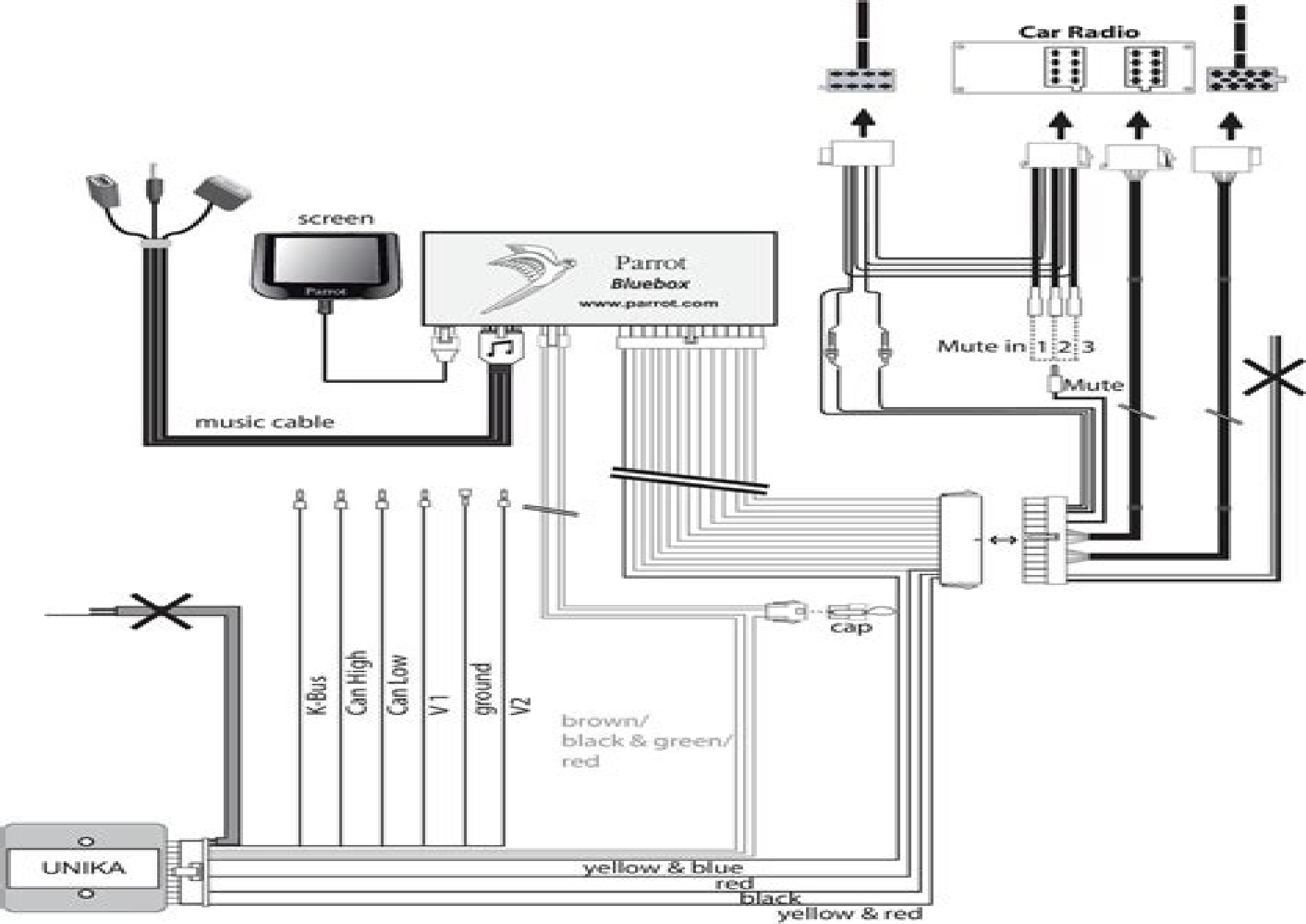
Parrot MKi9200
