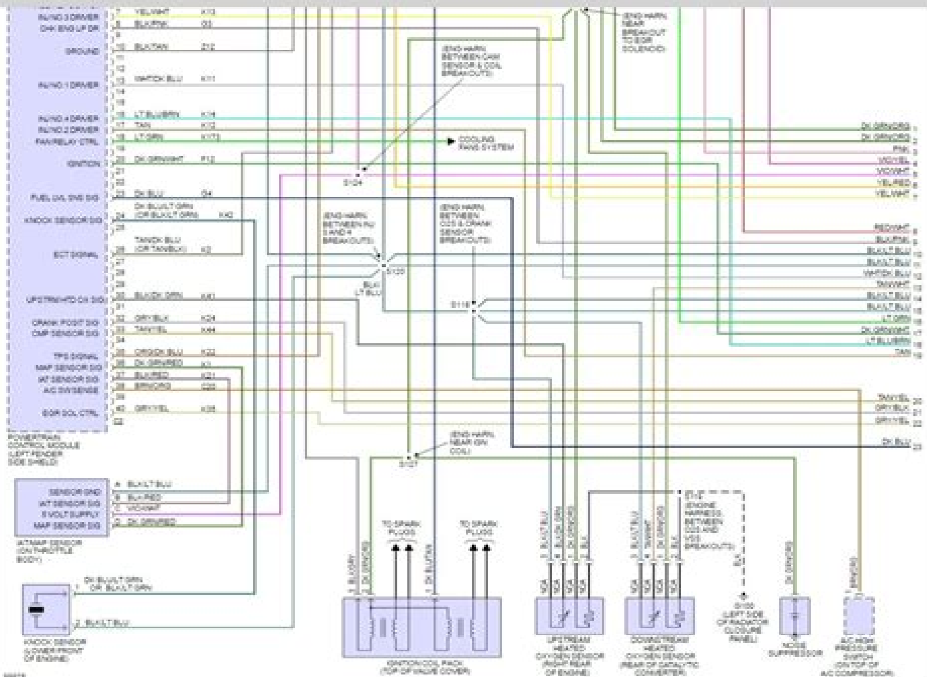
Fig 1 2.0L Engine Performance Circuits (1 of 3)
