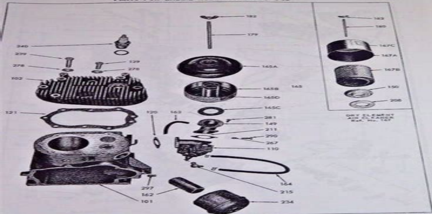
CRANKCASE, CYLINDER HEAD, CARBURETOR and AIR CLEANER GROUP
