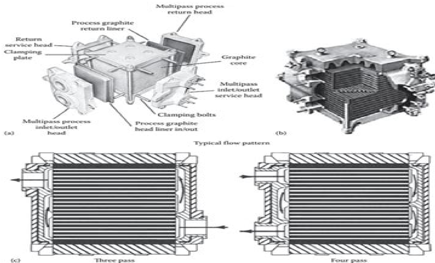
FIGURE 1.25 NK series multipass cubic graphite heat exchanger. (a) Construction details, (b) cut section, and (c) multipass flow pattern. (Courtesy of MERSEN, Paris La Défense, France.)
