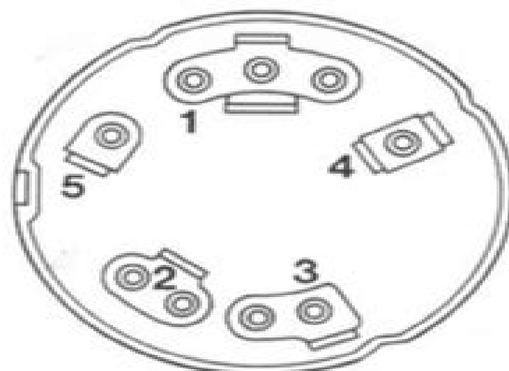
KEY SWITCH TERMINALS 5 POSITION SWITCH
