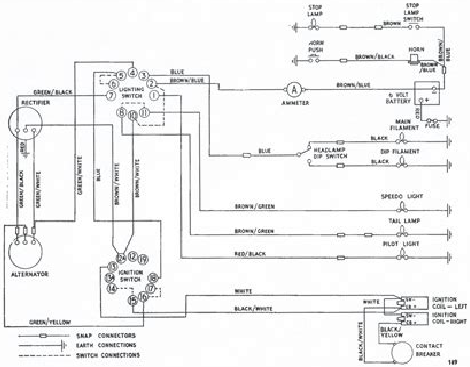
Fig. H22. Wiring diagram—Cell Ignition 6V models
