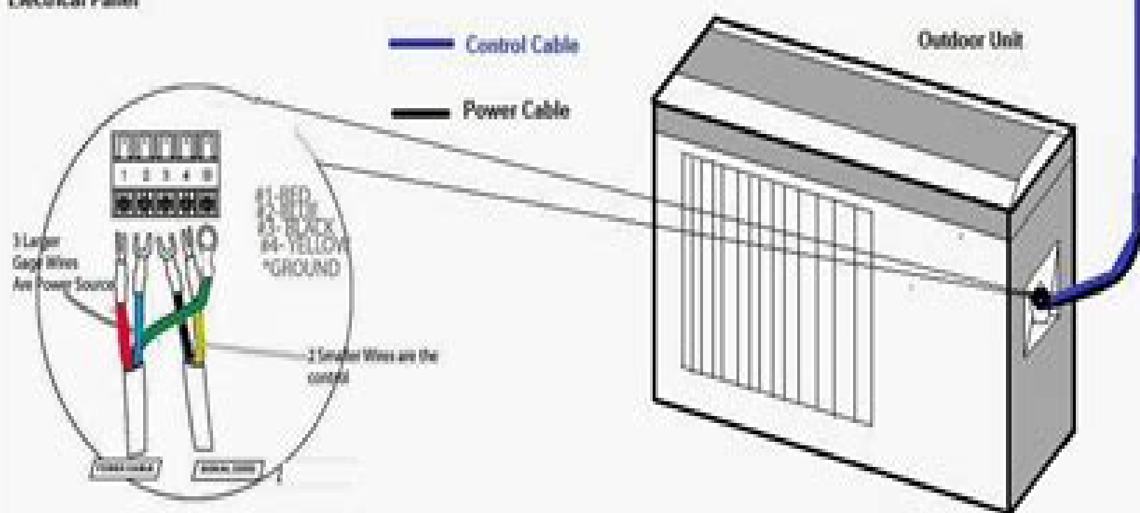
Electrical Panel
