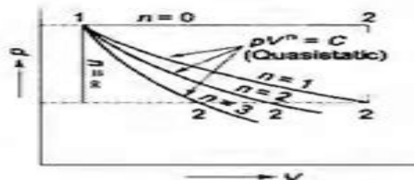
Fig. 3.10 Process in which pV^n = \text{constant}
