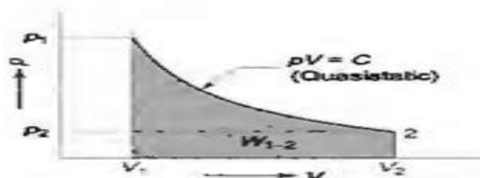
Fig. 3.9 Process in which pV = \text{constant}
