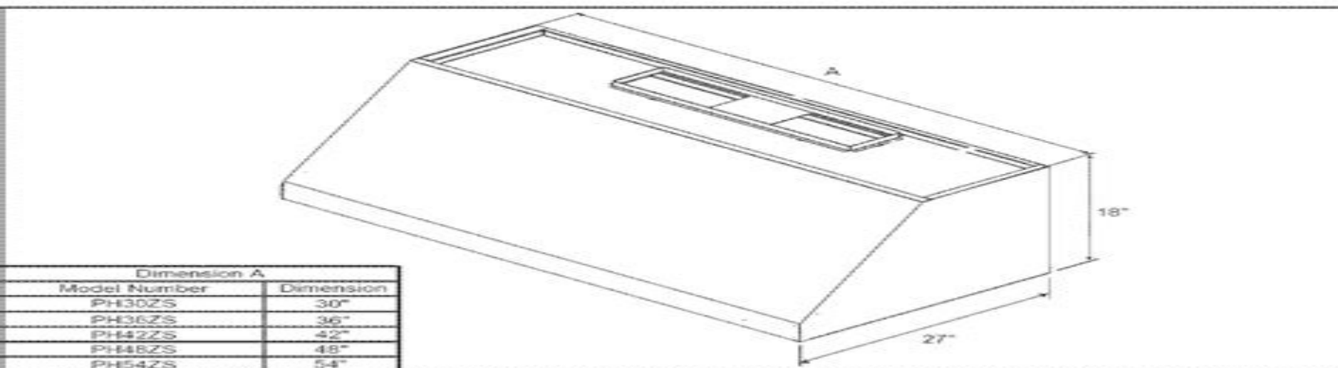
Figure 1b: Overall Dimensions
