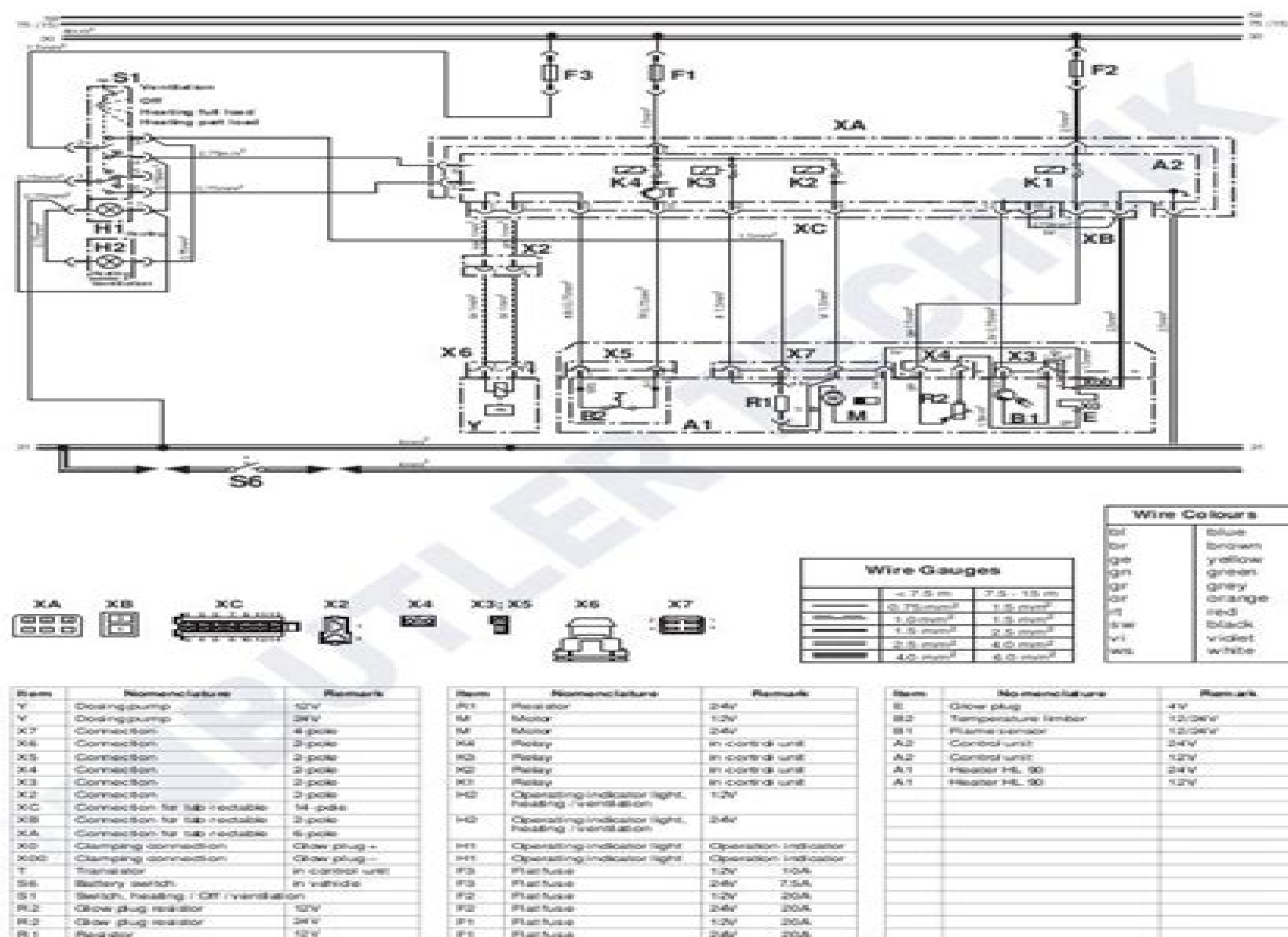
Fig. 702 Operation with Switch (Full Load - Part Load) and Ventilation
