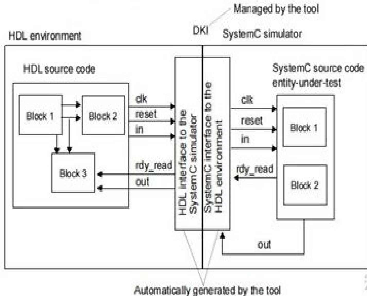
Figure 4-1 VCS DKI Communication of a Verilog Design Containing SystemC Modules
