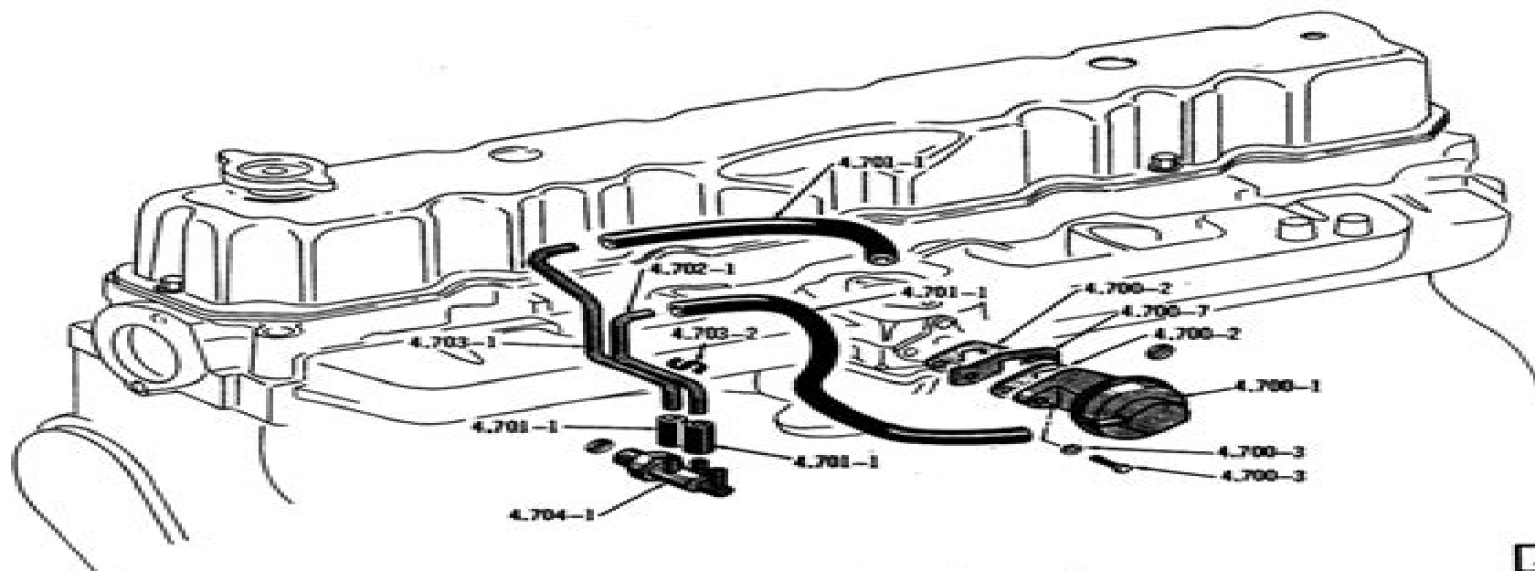
EXHAUST GAS RECIRCULATION . . . SIX
