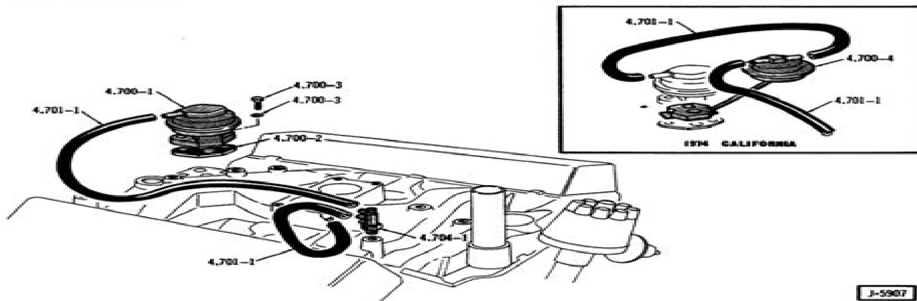
EXHAUST GAS RECIRCULATION . . . V8
