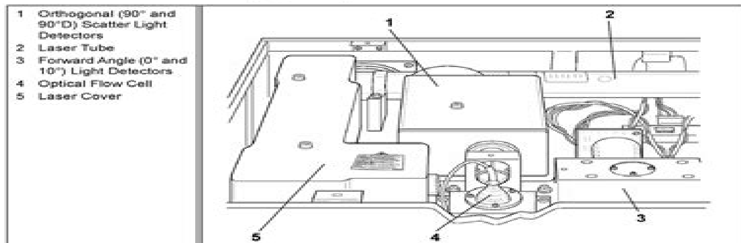
Figure 3.1 Optical Bench
