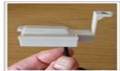
Gas pulse sensor- type B (Shown before attaching to a gas meter)
