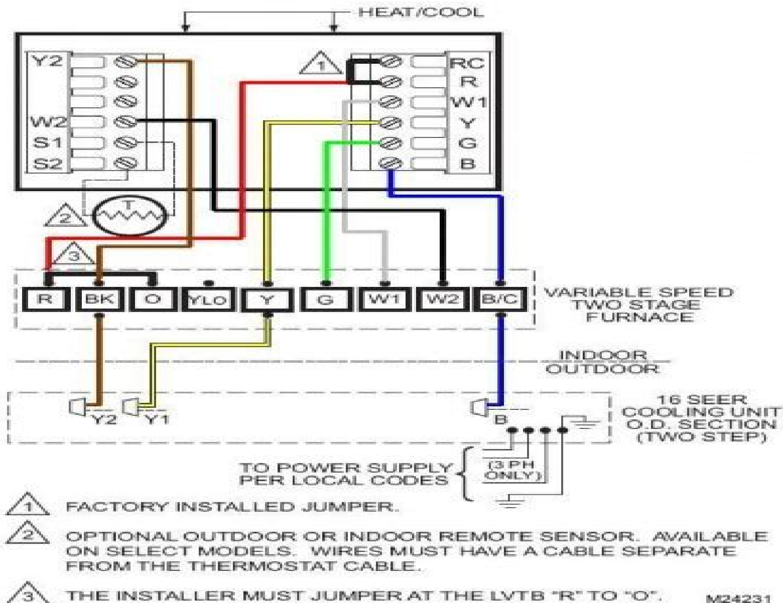
Fig. 8. Typical hookup of two-stage indoor and two-step scroll cooling unit in a single transformer system (2H/2C or 2H/1C or 1H/2C).
