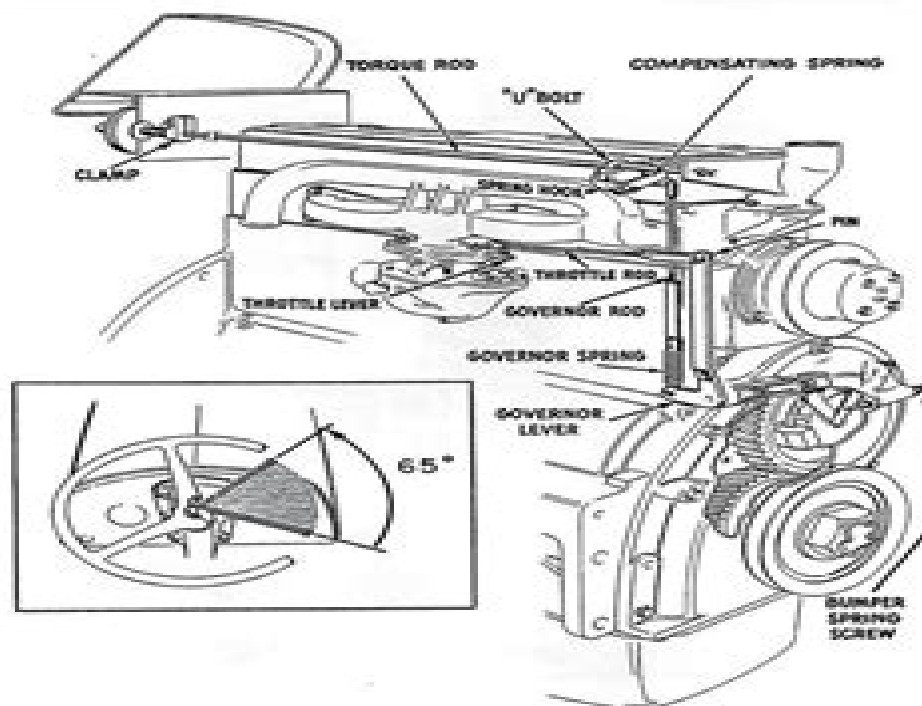
Fig. 46 Governor Linkage
