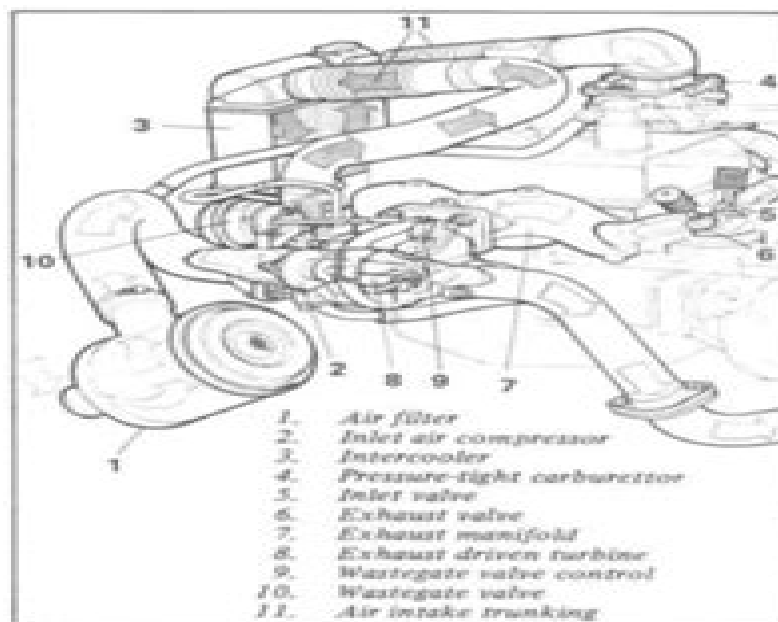
Fig. B:6 Details of the turbocharging system - 807 type
