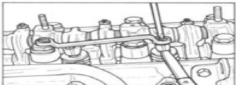
Fig. B:7 Checking/adjusting valve clearance - OHC
