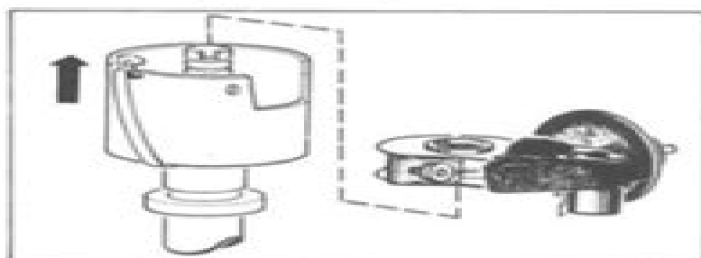
Fig. B:10 Lifting out "cassette" type points assembly
