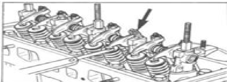
Fig. B:5 Checking/adjusting valve clearance - OHV
