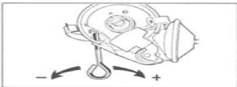
Fig. B:9 "Cassette" type contact points adjustment
