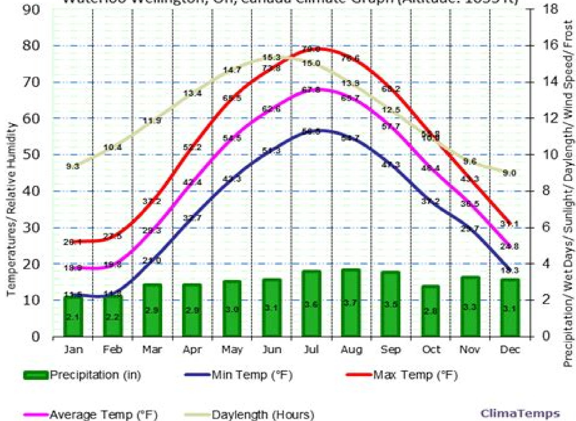
Waterloo Wellington, On, Canada Climate Graph (Altitude: 1055 ft)
