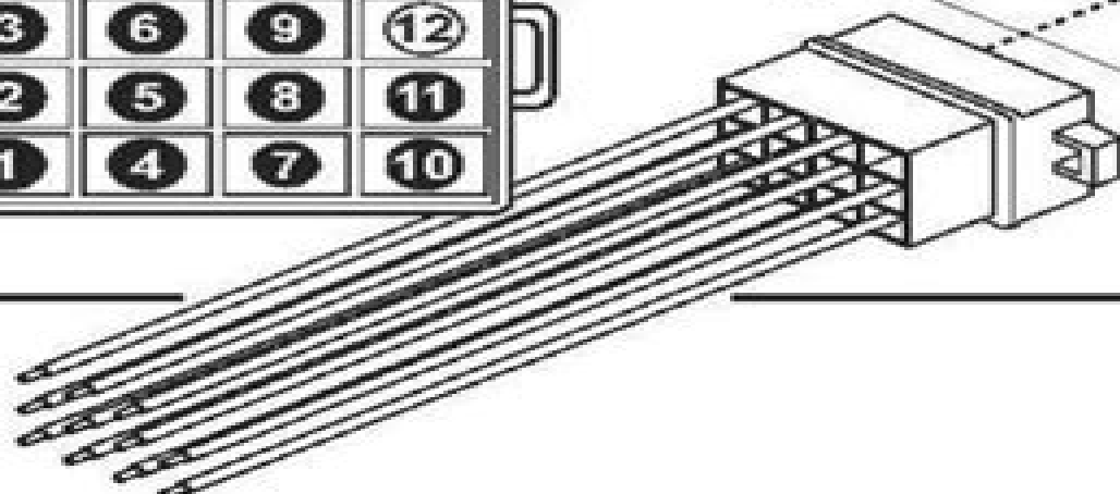
INPUT CONNECTOR (REAR VIEW)
