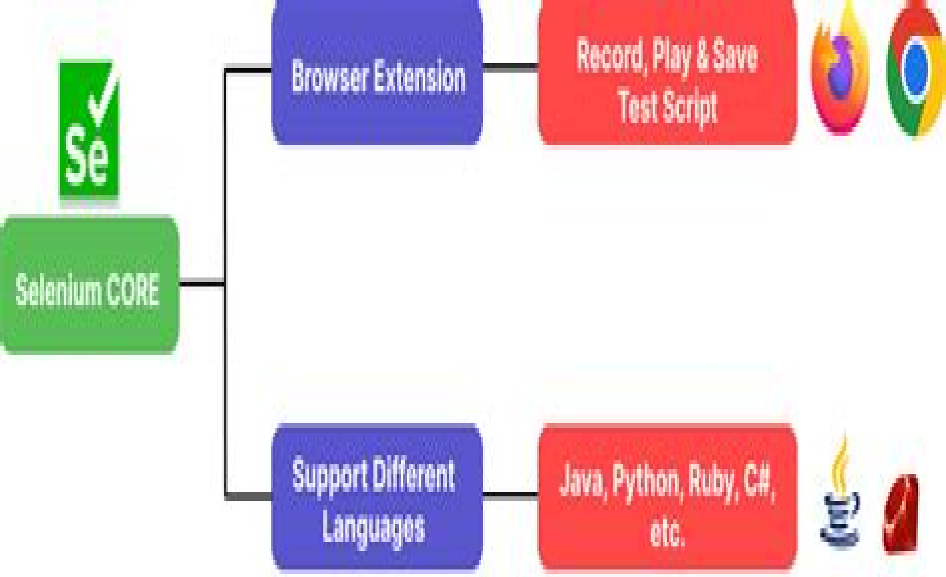
Selenium Architecture
