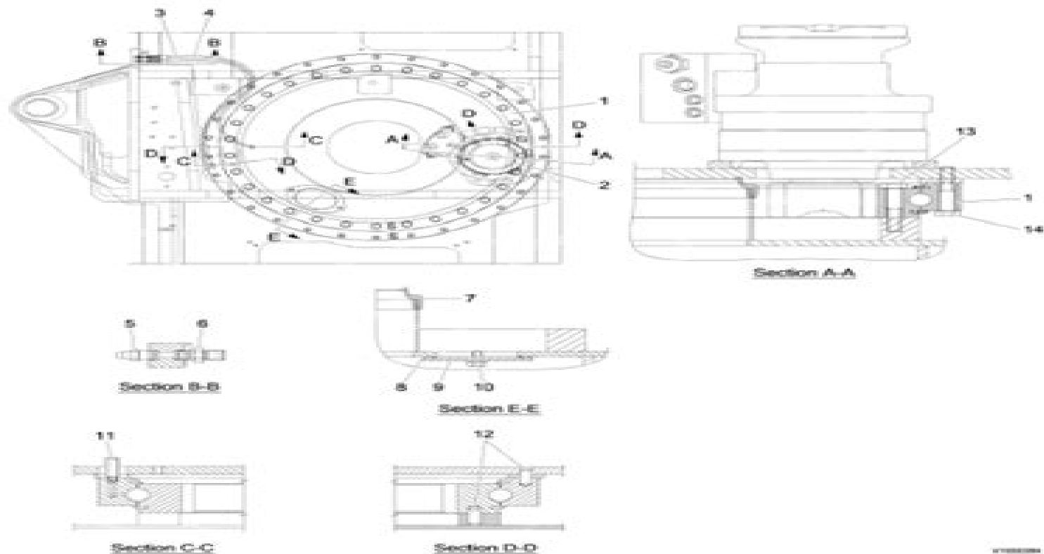
Figure 898 Slew ring gear, structure
