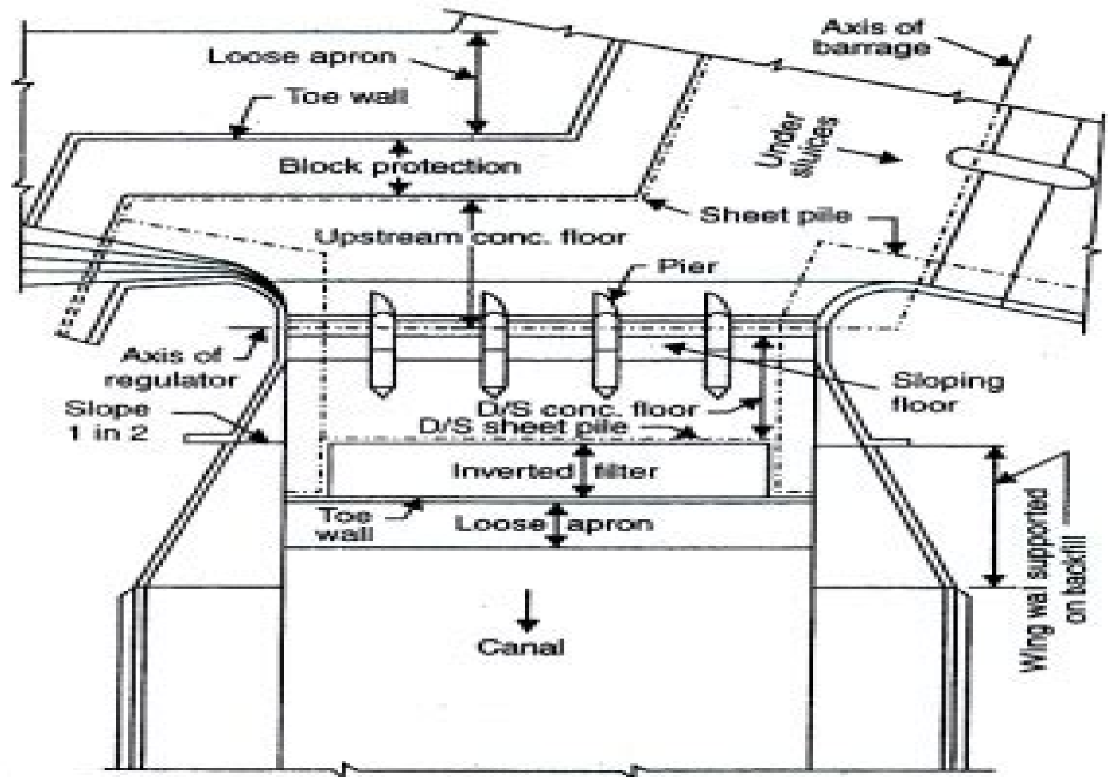
Figure: Typical plan of a head regulator (6)
