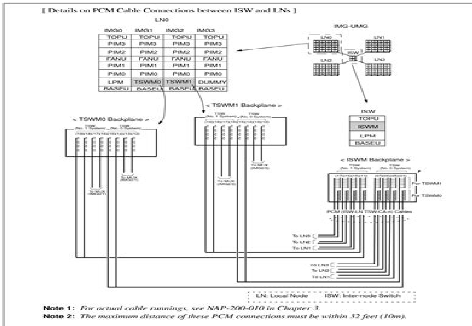
Figure 2-5 Details on PCM Cable Connections between ISW and LNs
