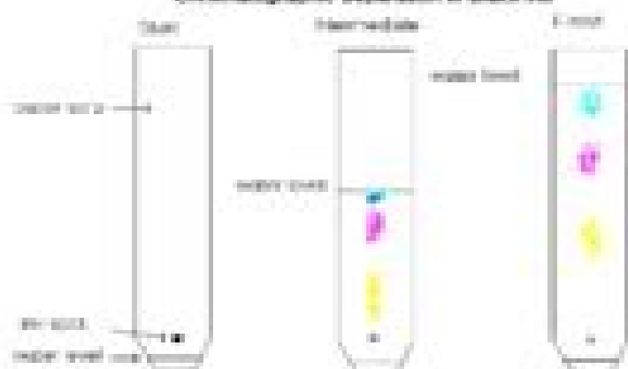
Chromatography: Separation of Black Ink
